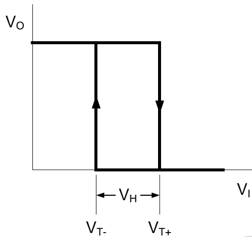
Figure 6. Transfer characteristics
